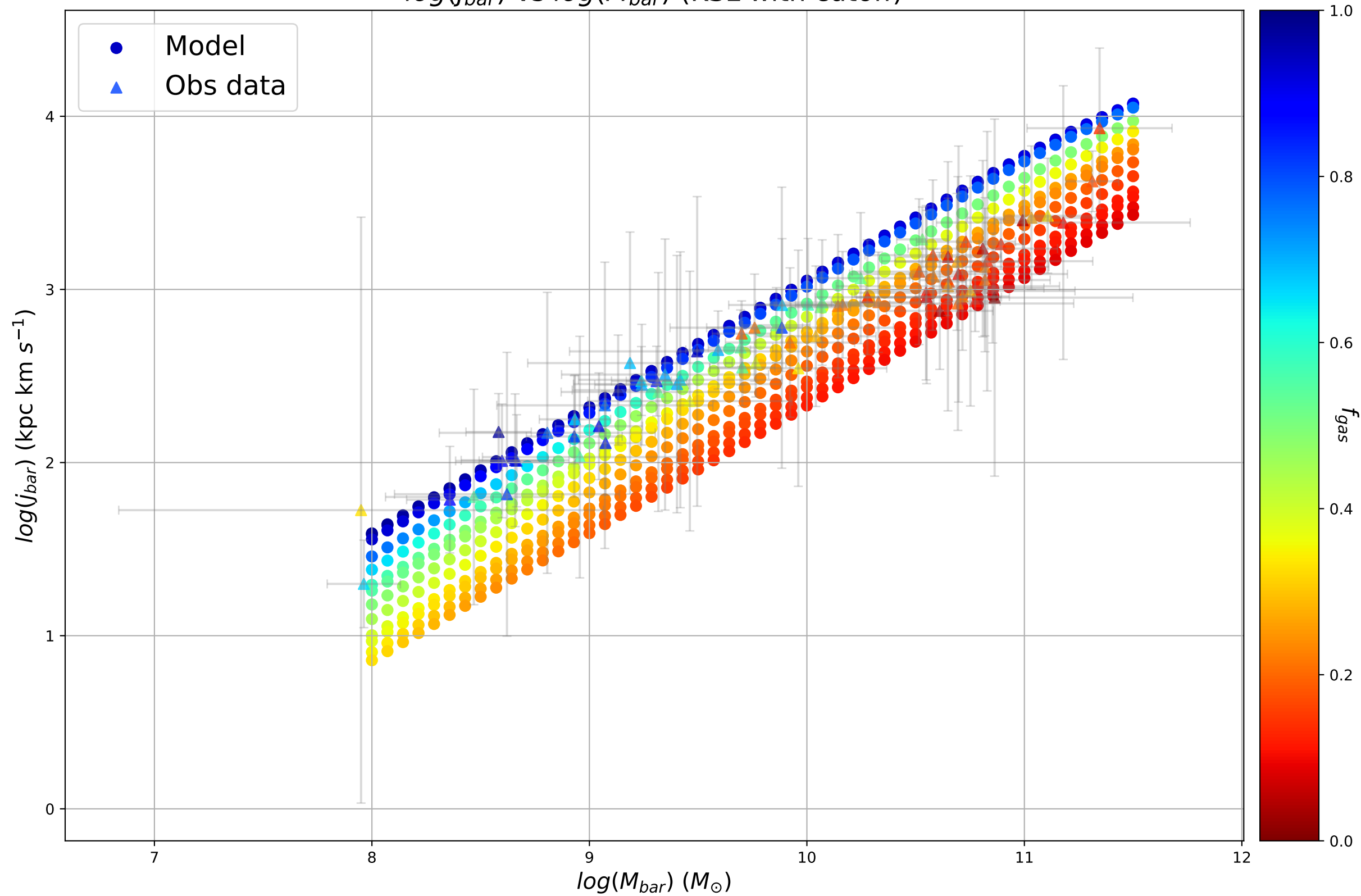
\log(j_{bar}) vs \log(M_{bar}) (KSL with cutoff)
